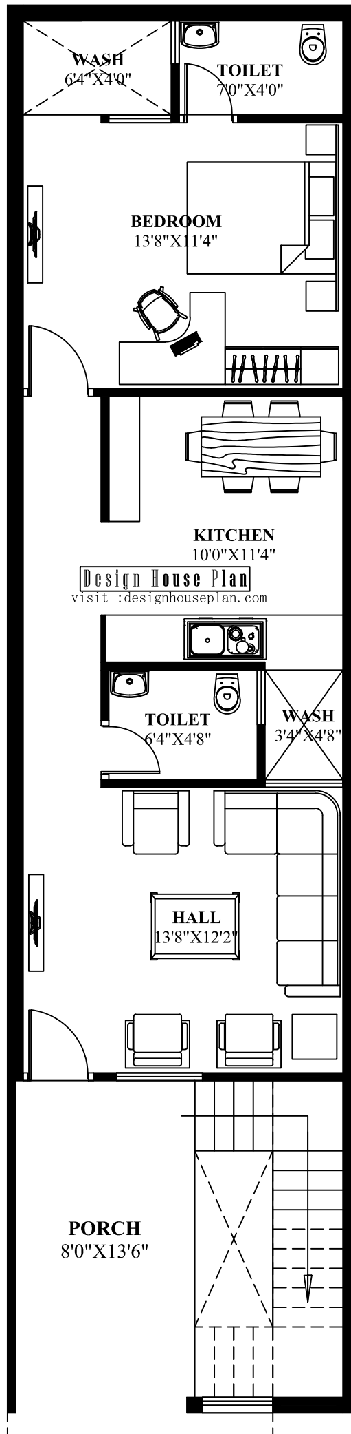
15'0"X60' ,1BHK GROUND FLOOR
