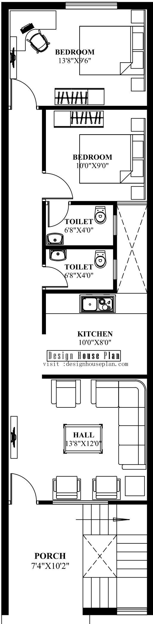
15'0"X60' ,2BHK GROUND FLOOR
