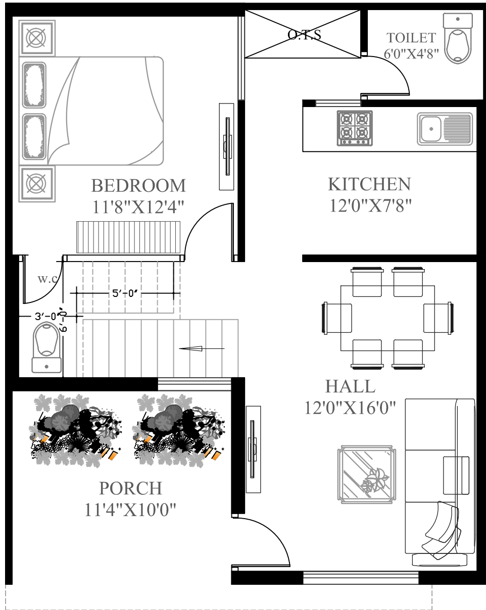
25'X30' DUPLEX, 3BHK GROUND FLOOR
