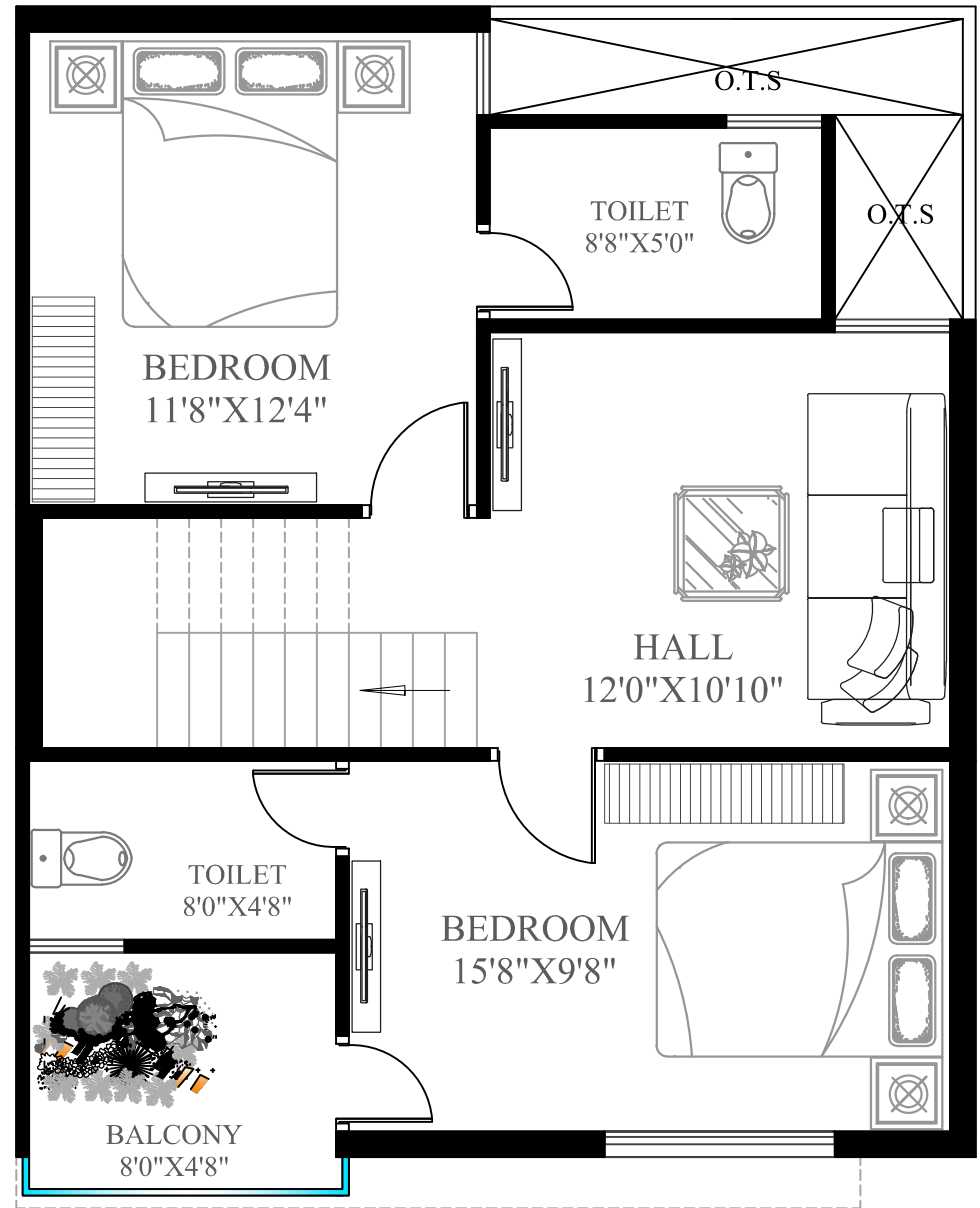
25'X30' DUPLEX, 3BHK FIRST FLOOR
